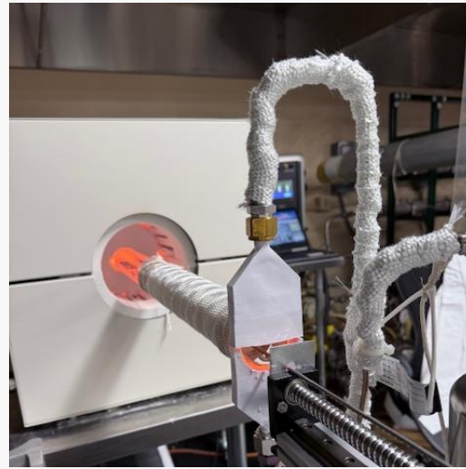
Mimic incinerator
