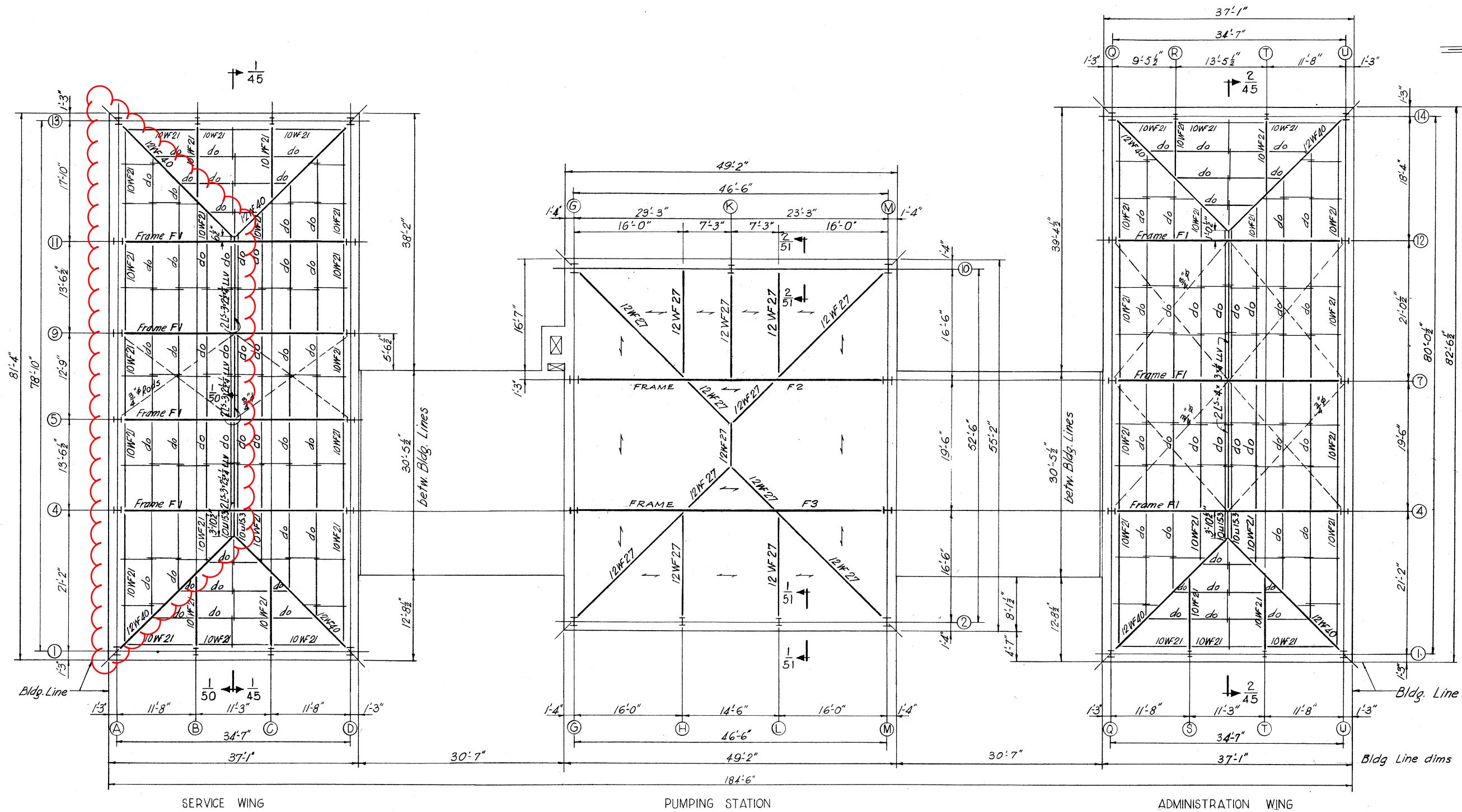
ROOF FRAMING PLAN SCALE 1/8" = 1'-0"
